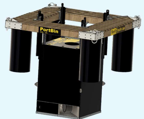
PortBin Tide XL Weight 615 kg Collect 1000 l 2200 2400 2400
